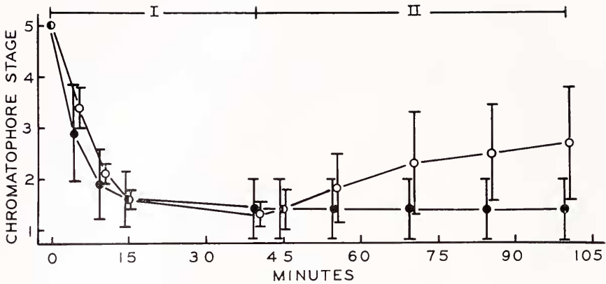
FIGURE 3. Effect of colchicine on ionophore A23187-mediated pigment movement in ovarian erythrophores of Palaeomonetes pugio . Ovaries were removed and bisected, the experimental halves (dots) being pre-incubated in saline containing 25 mM colchicine and the controls (circles) in saline alone. After 30 min (at t=0 min), the ionophore was added to all incubation media to a concentration of 25 \mu M, starting phase I. Forty minutes later, the test solutions were replaced with Ca^{++} -free/5 mM EGTA saline containing (dots) or lacking (circles) 25 mM colchicine, starting phase II. Five ovaries were used.
